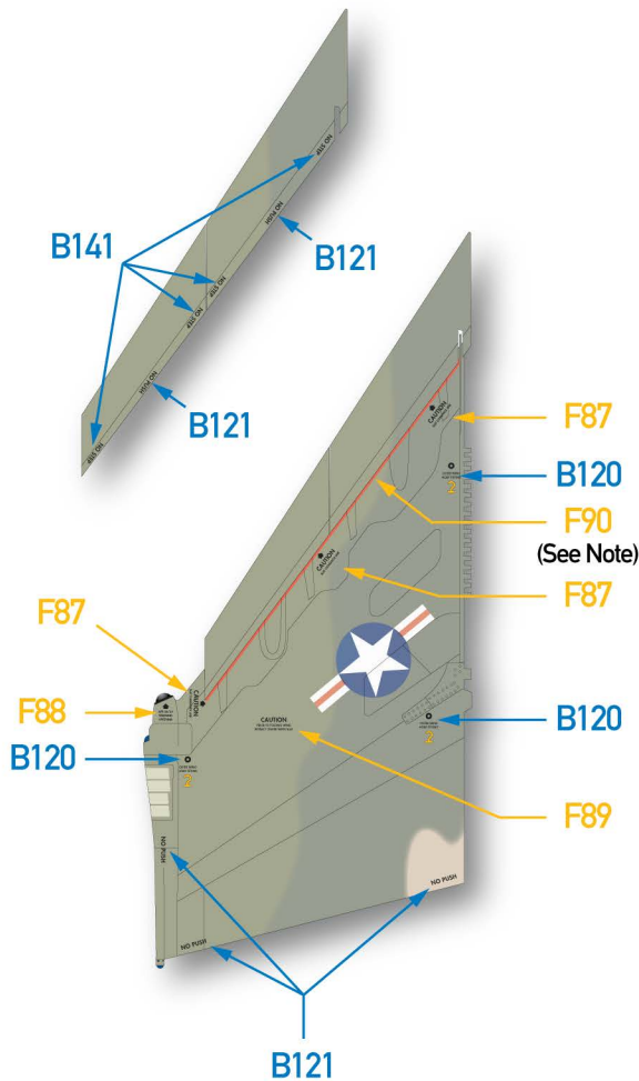
Outboard slat upper surface (right side markings identical)
